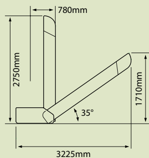
Conveyor unit
